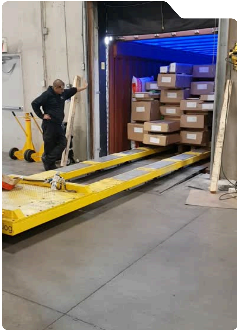
PNEUMATIC FORK FOR MANUAL LOADING AND UNLOADING
